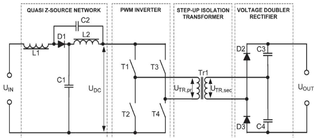
Fig. 1. Simplified power circuit diagram of the proposed converter.
