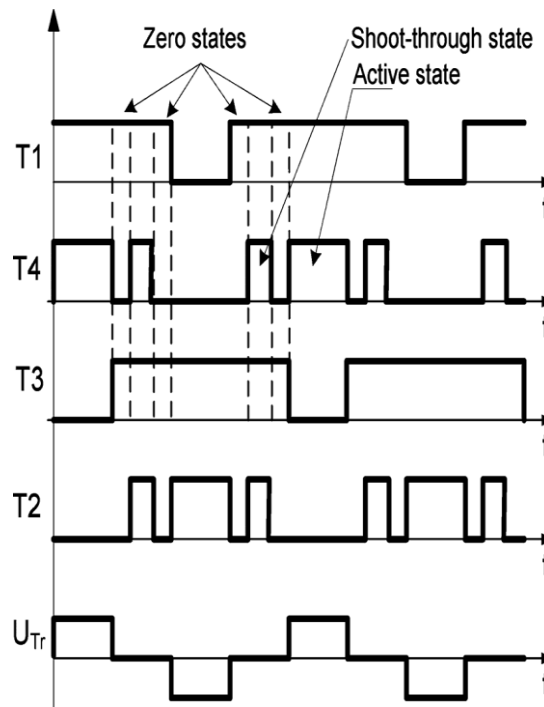
Fig. 2. Generation of PWM signals with shoot-through during zero states.
