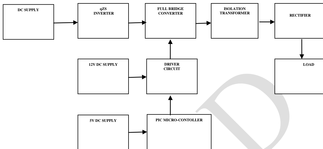
Fig.5 Block diagram of the proposed system
