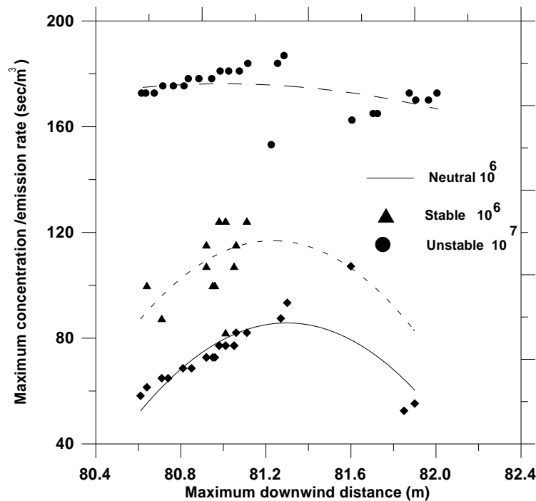
Fig. 1. Variation of the maximum concentration over emission rate ( C_{\max}/Q ) with the maximum downwind distances ( x_{\max} ) in all stabilities.
