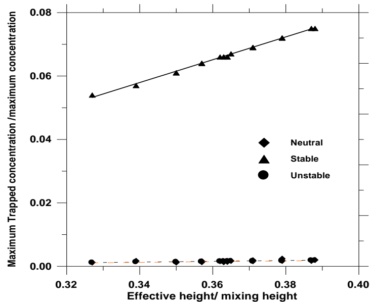
Fig. 2. The variation the ratio of ground-level trapping to non-Gaussian concentration via non-dimensional distance.
