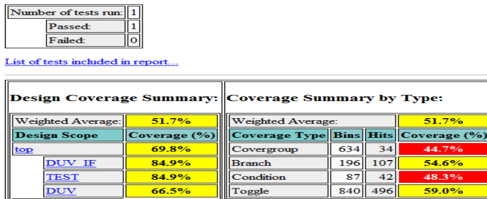
Figure 4: Functional Coverage of Router Random Test cases
