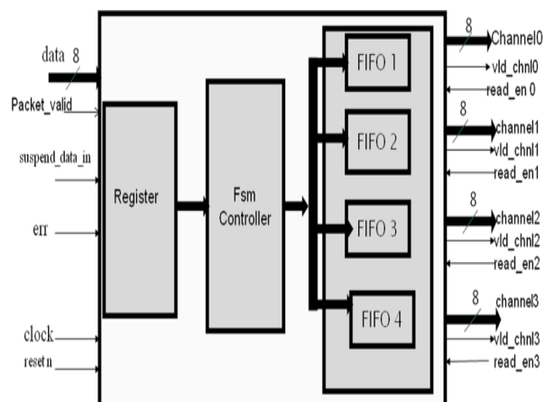
Figure 2: Internal Structure of Protocol
