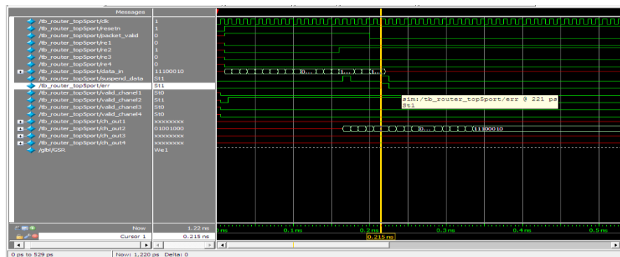
Figure 7: Simulation Results of Router Protocol
